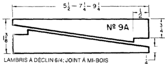
6/4 BEVEL SIDING; SHIPLAP JOINT
