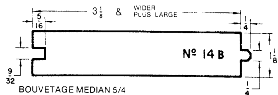
5/4 CENTRE MATCHED
