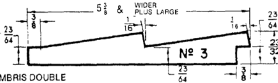
LAMBRIS DOUBLE
