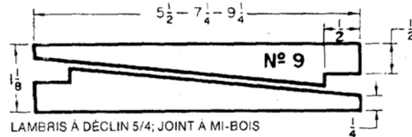
5/4 BEVEL SIDING; SHIPLAP JOINT
