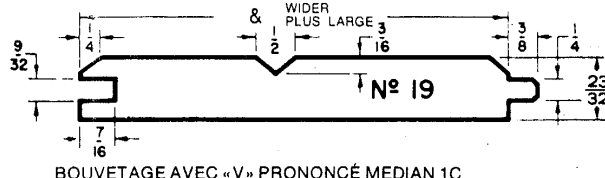
CENTRE V MATCH 1S WIDE V
