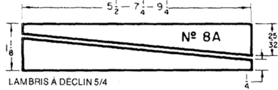
5/4 BEVEL SIDING
